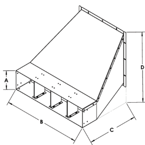
Transition
