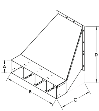
Transition
